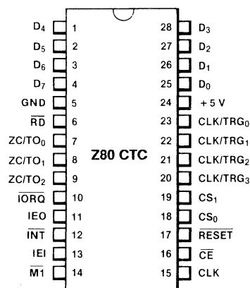
Figure 22a. Pin Assignments
