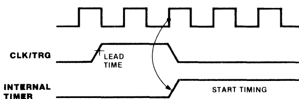
Figure 11. Timer Mode Timing
