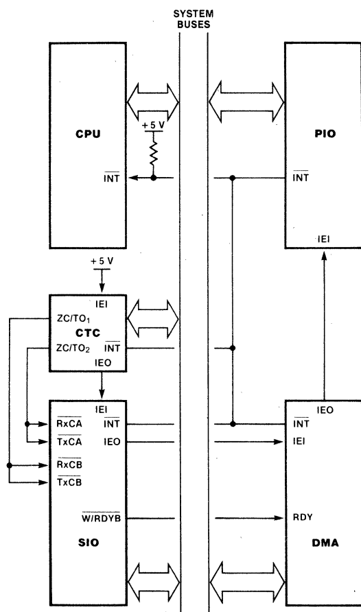
Figure 8. A Typical Z80 Environment
