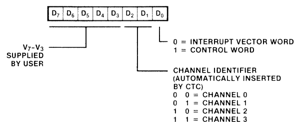
Figure 7. Interrupt Vector Word
