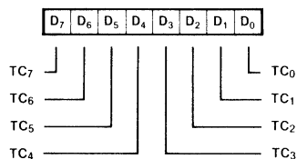
Figure 6. Time Constant Word
