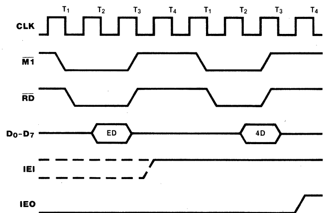
Figure 15. Return From Interrupt Timing
