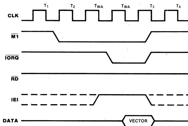
Figure 14. Interrupt Acknowledge Timing
