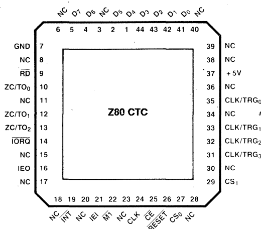
Figure 2b. 44-pin Chip Carrier, Pin Assignments
