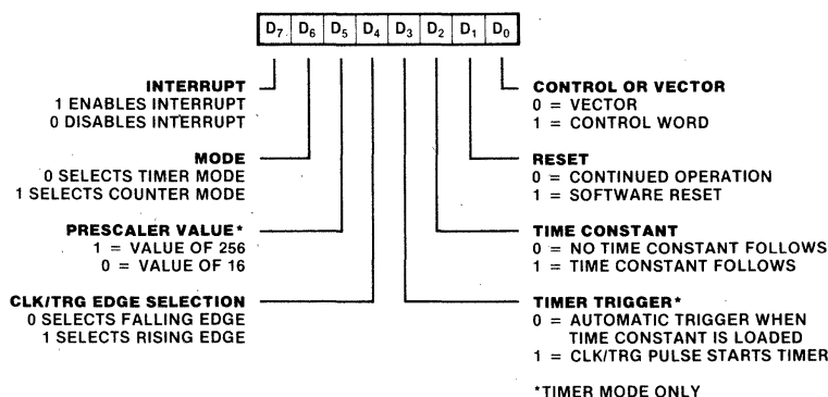
Figure 5. Channel Control Word
