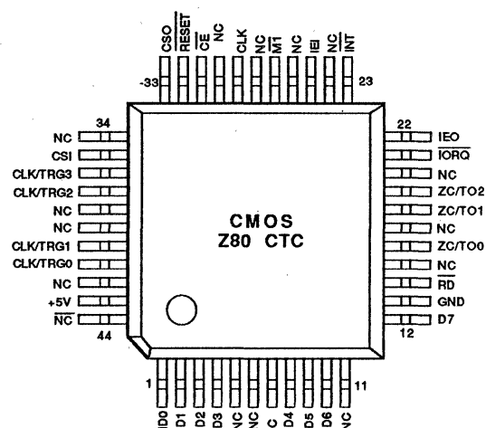
Figure 2c. 44-Pin Quad Flat Pack Pin Assignments
