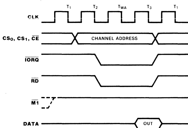
Figure 9. Read Cycle Timing
