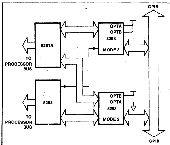
Figure 4. Talker/Listener/Controller Configuration
