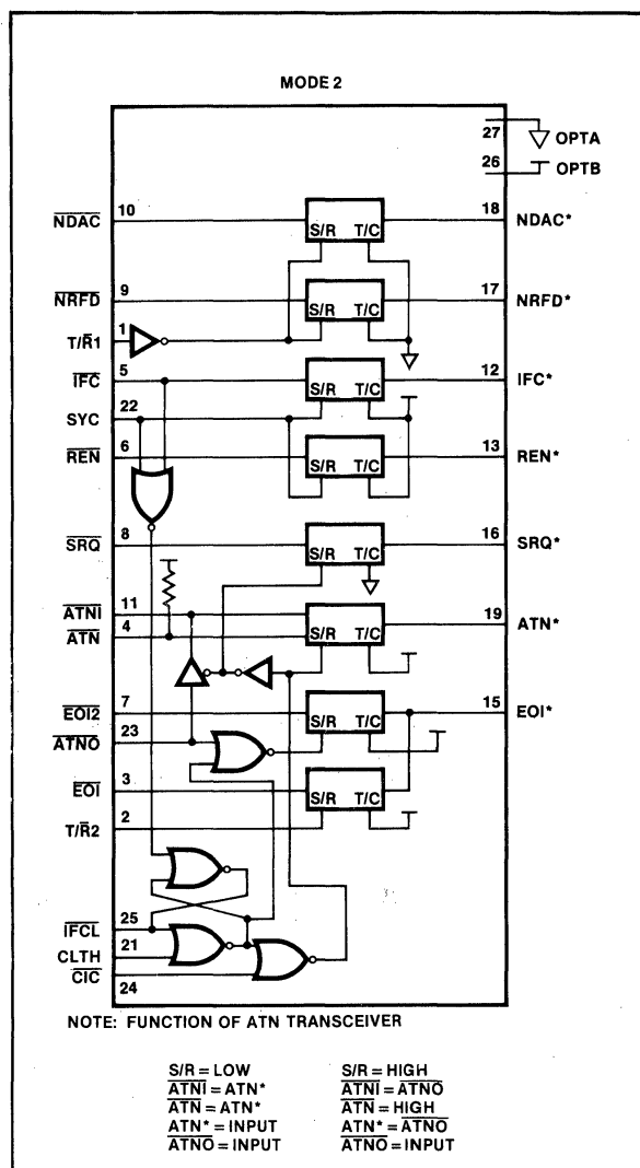
Figure 7. Talker/Listener/Controller Control Configuration
