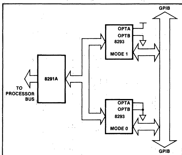
Figure 3. Talker/Listener Configuration
