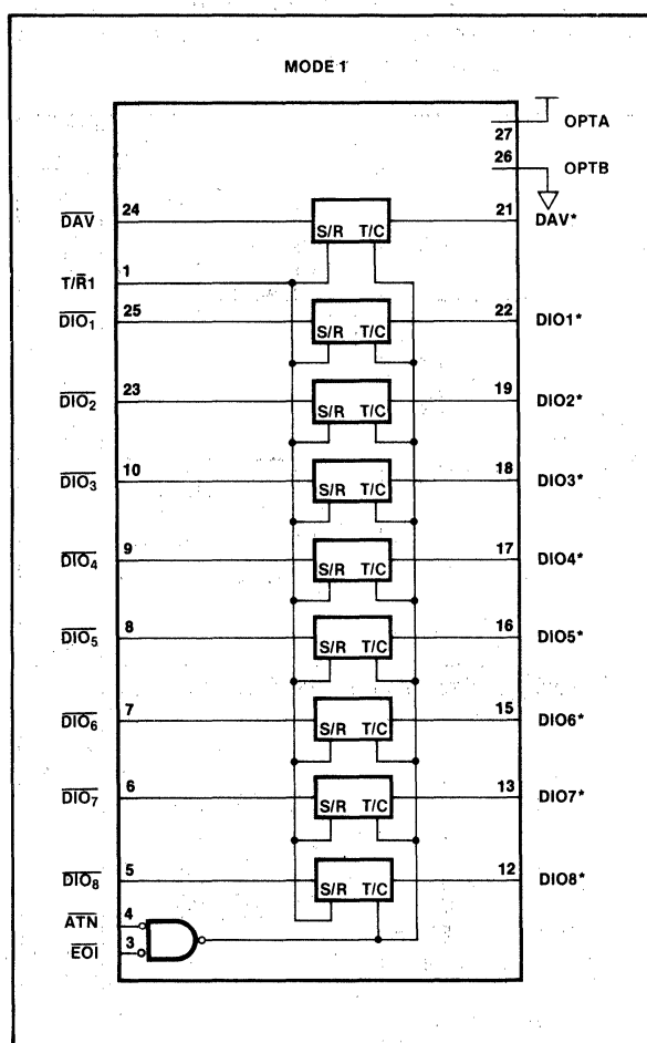
Figure 6. Talker/Listener Data Configuration
