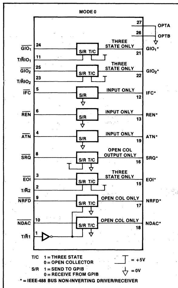
Figure 5. Talker/Listener Control Configuration
