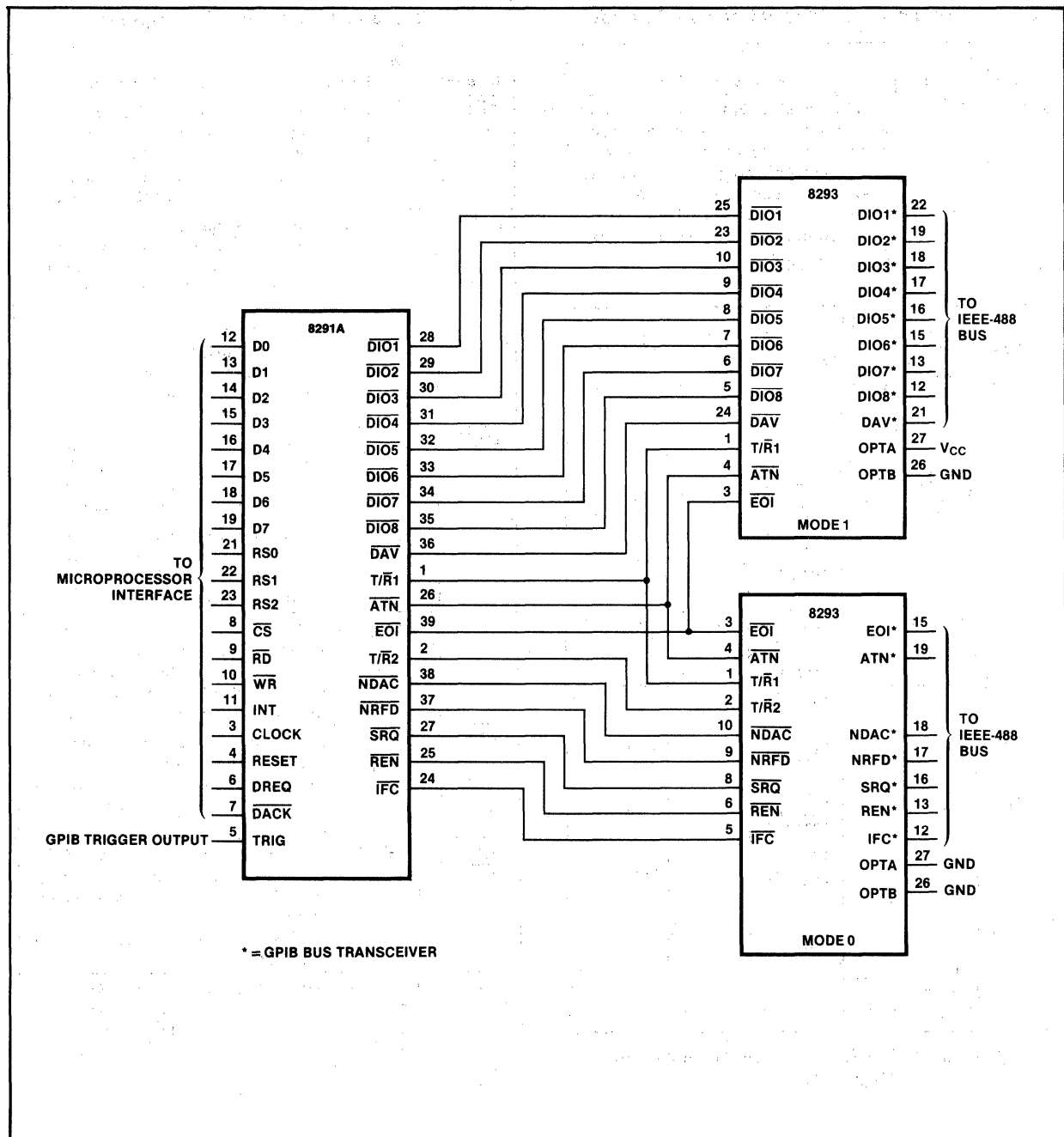
Figure 9. 8291A and 8293 System Configuration
